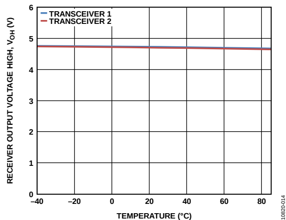
Figure 5. Receiver Output Voltage High vs. Temperature
