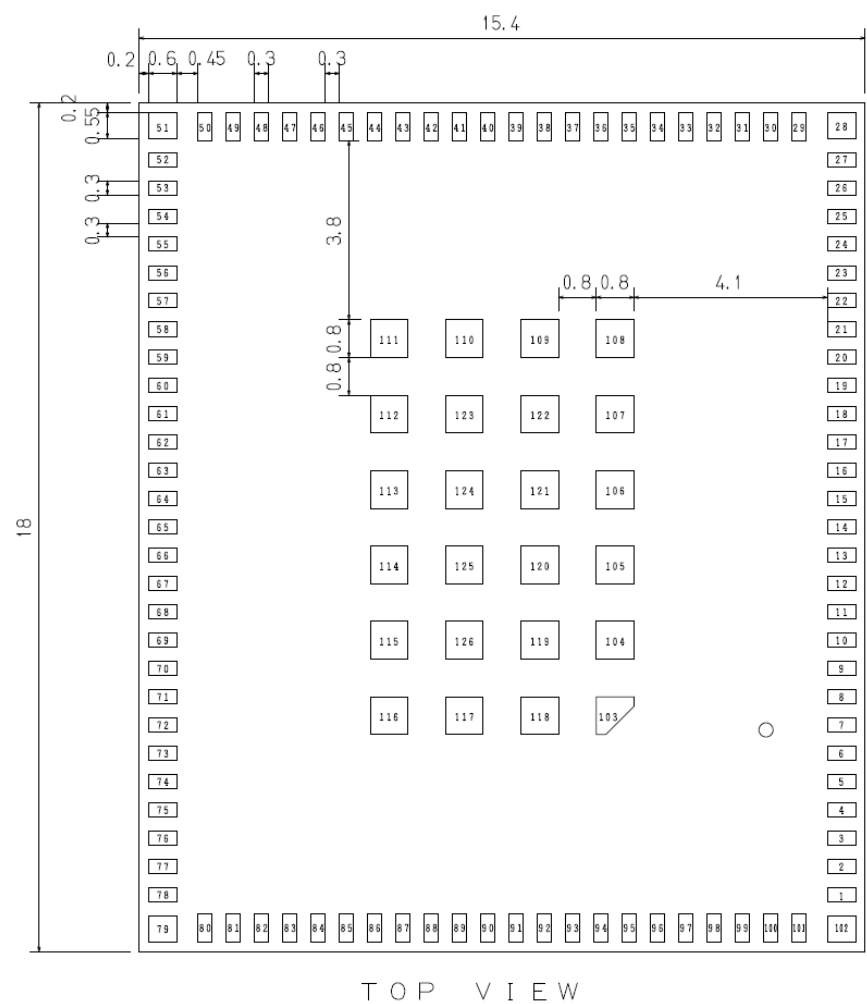
Figure 2.2 Module Footprint Top View (Unit: mm)
