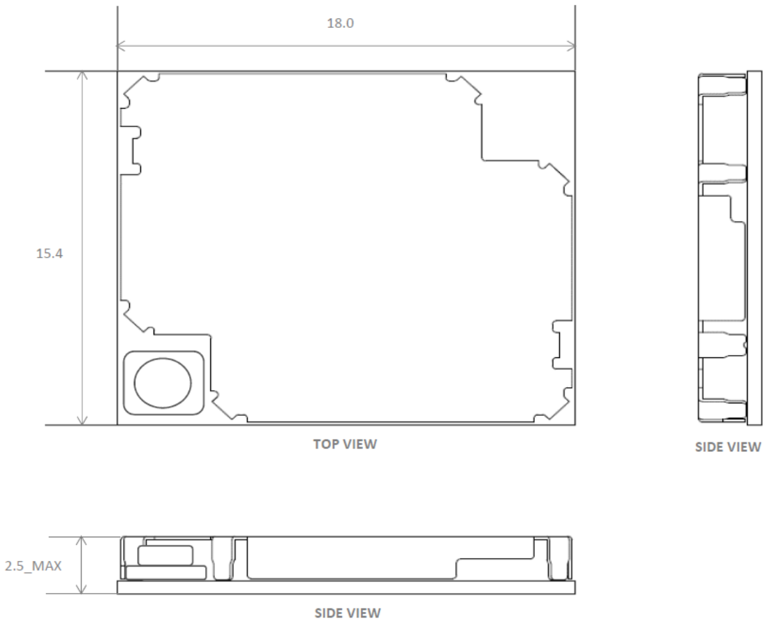
Figure 2.1 Module Top and Side View (Unit: mm)
