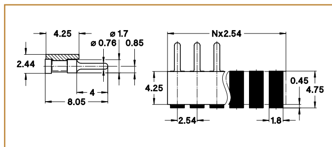
Pin connector 8MM-11-0NNN-02-279
