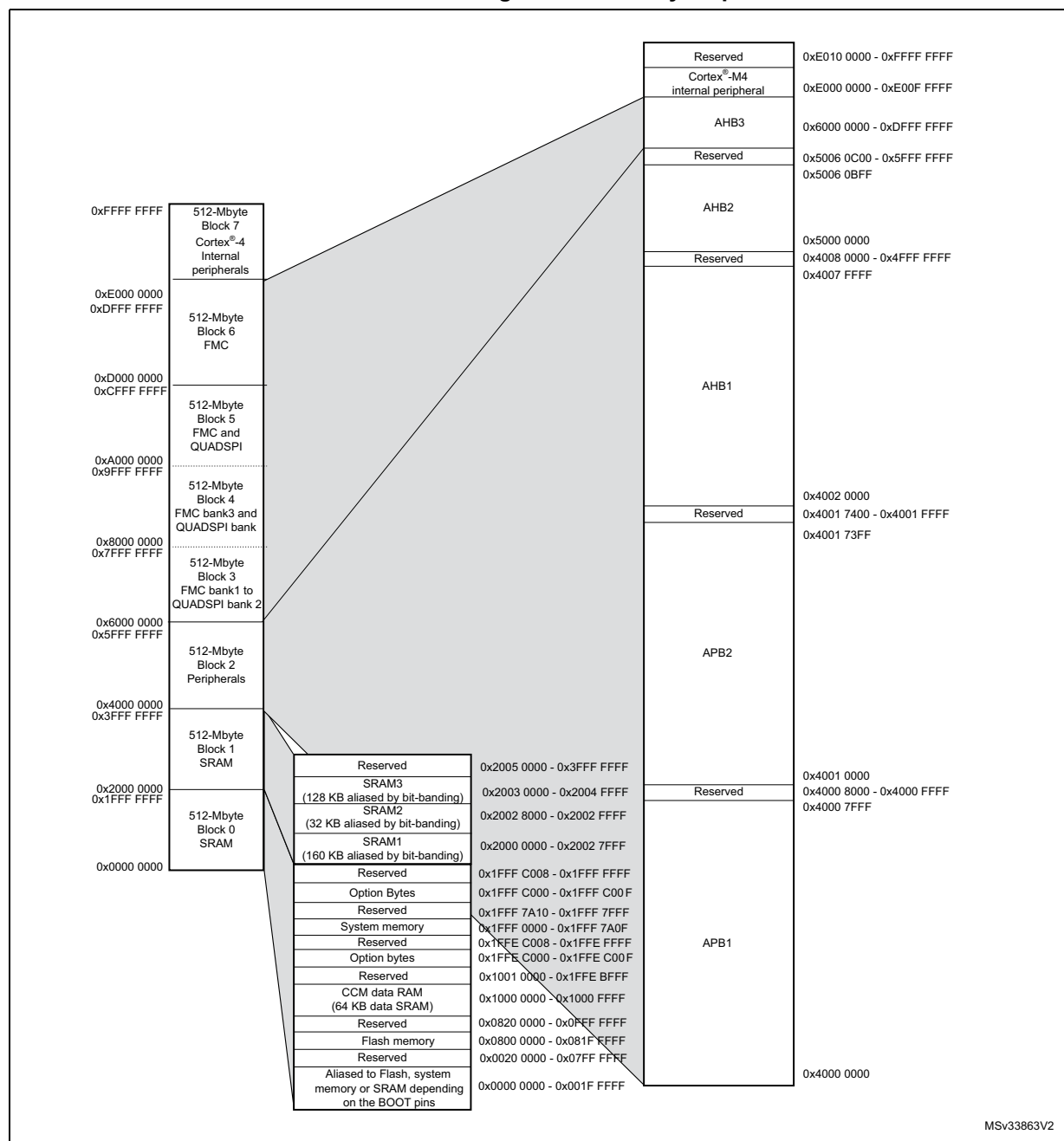
Figure 21. Memory map
