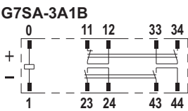
Terminal Arrangement/ Internal Connection Diagram (Bottom View)
