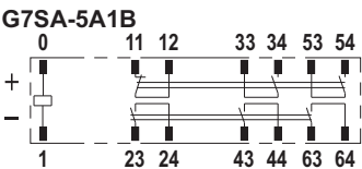
Terminal Arrangement/ Internal Connection Diagram (Bottom View)
