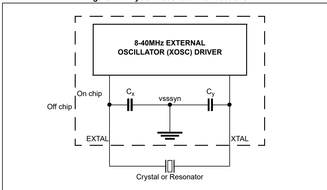
Figure 11. Crystal/Resonator Connections
