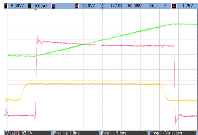
Figure 4: Typical Waveforms for V_{IN} = 48 \text{ V} to 5 \text{ V}/25 \text{ A} (300 kHz) Buck converter CH1: ( V_{PWM} ) Input logic signal – CH2: ( I_{OUT} ) Output inductor current – CH3: ( V_{IN} ) Input voltage – CH4: ( V_{OUT} ) Switch node voltage
