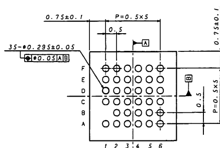
Figure 3 External dimensions (Unit:mm)
