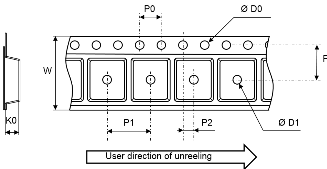
Figure 23. Tape and reel outline
