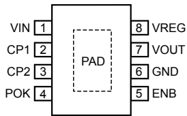
Pinout Diagram
