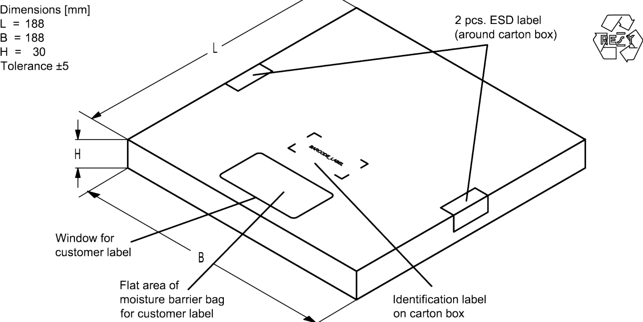
Figure 15: Drawing of folding box for reel with diameter of 180 mm.
