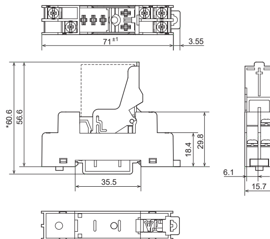
External dimensions
