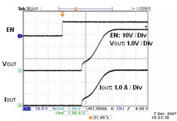
Figure 17. Start Up Waveform (VIN= 12V VOUT= 3.3V L= 22μH CSS= 0.1μF IOUT= 0A)
