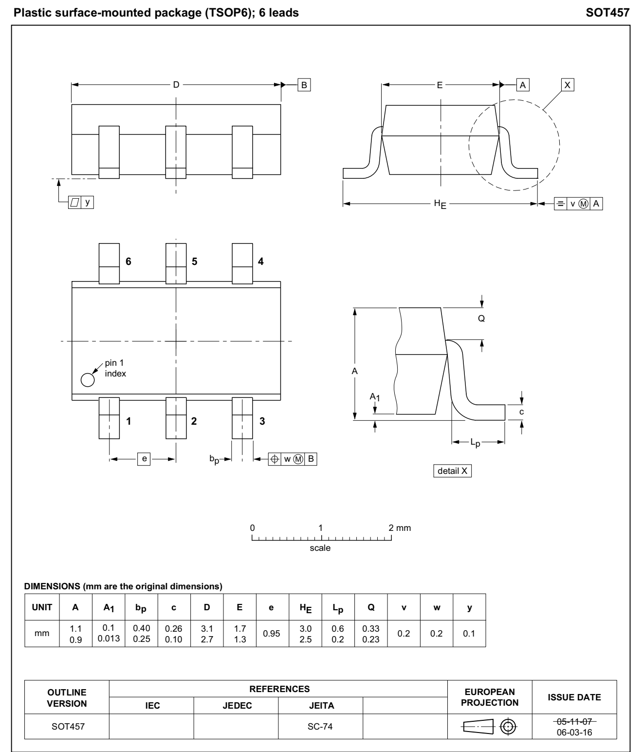
Fig 15. Package outline SOT457 (TSOP6)
