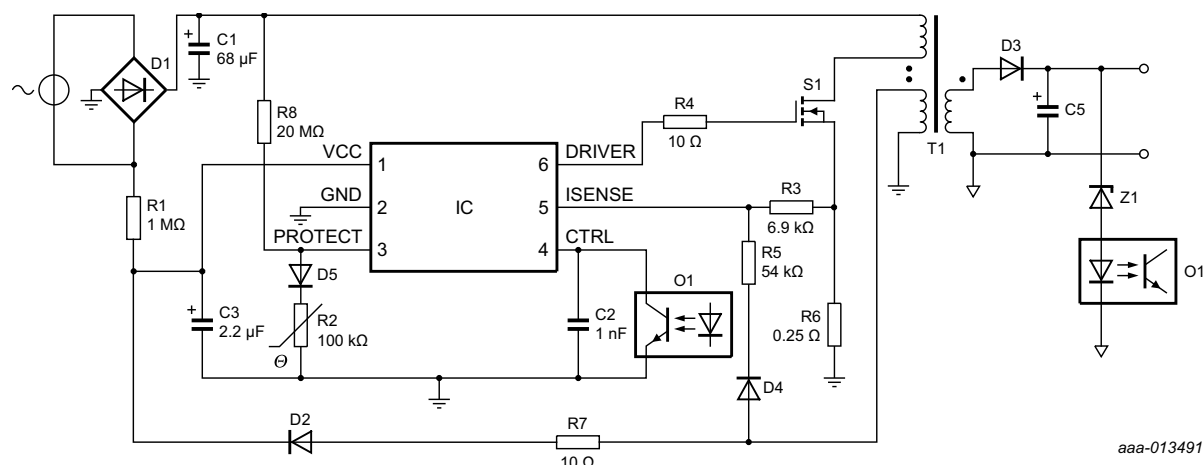
Fig 14. TEA1832TS application diagram
