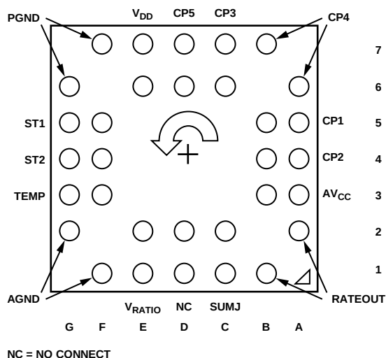
Figure 3. Pin Configuration
