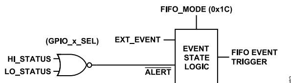
Figure 83. FIFO Event Detection Logic
