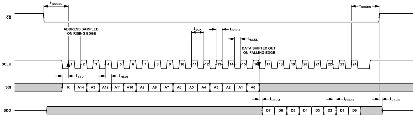
Figure 68. Configuration SPI Timing, Data Read Frame, 16-Bit Instruction Mode (Default)
