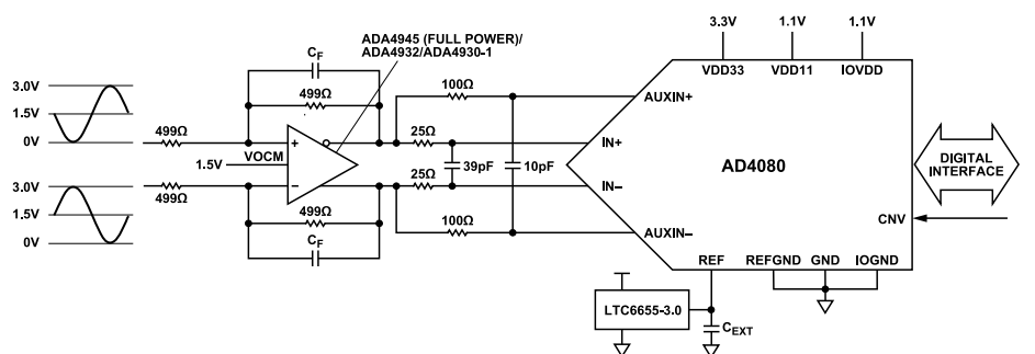
Figure 43. AD4080 Typical Applications Diagram, Fully Differential Amplifier
