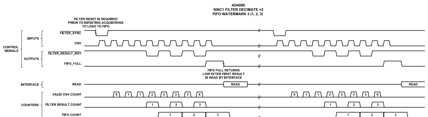
Figure 97. Description of Filter Timing with FIFO
