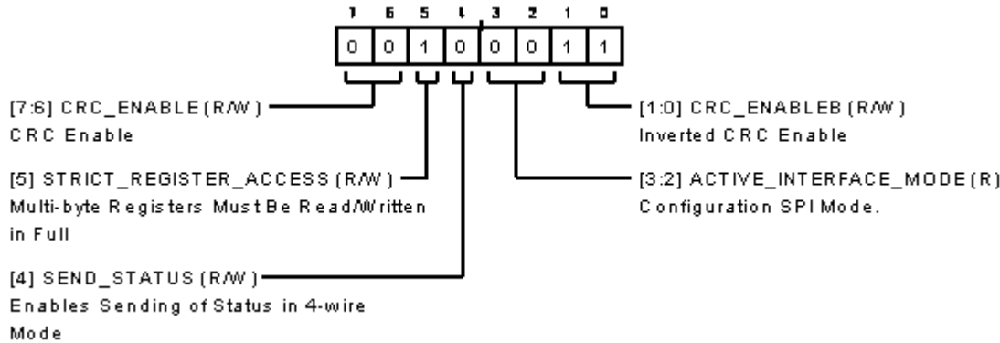
Figure 121. Interface Configuration C Register
