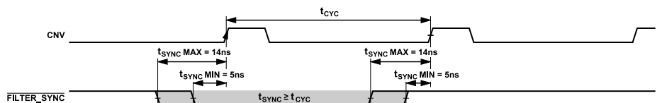
Figure 96. Filter Reset Timing
