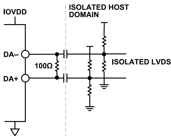
Figure 76. Isolated LVDS
