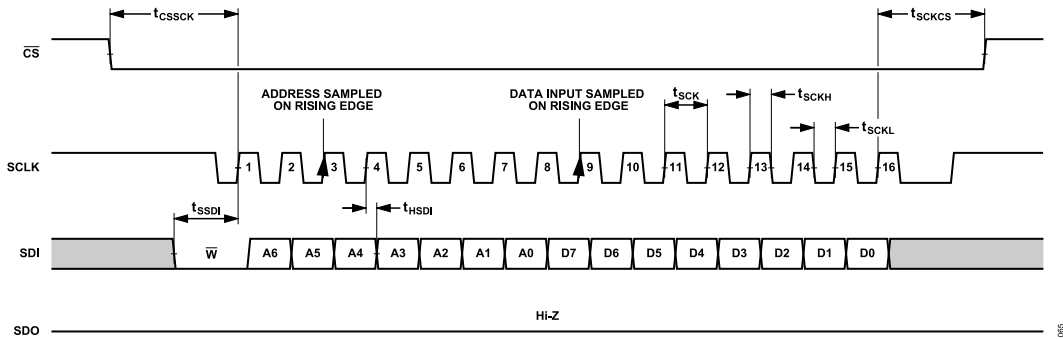
Figure 66. Configuration SPI Timing, Data Write Frame, 8-Bit Instruction Mode, Single 8-Bit Register
