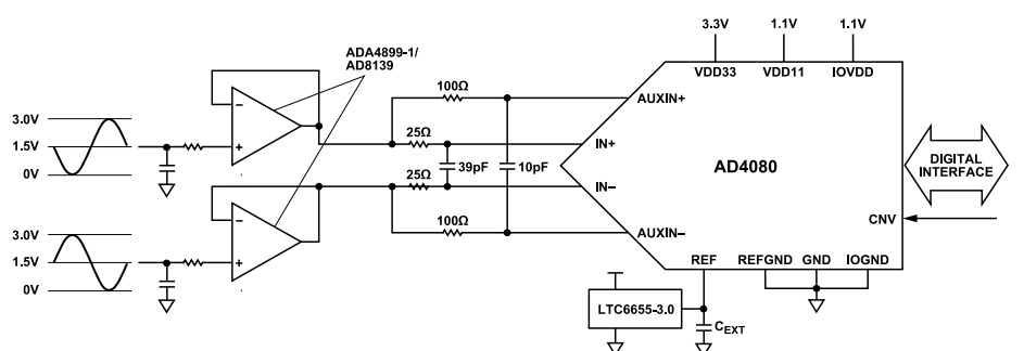
Figure 44. AD4080 Typical Applications Diagram, Single Op-Amp Drivers
