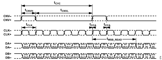
Figure 75. Continuous Conversion Timing, LVDS Data Interface, Dual Data Lane, Self Clock Mode
