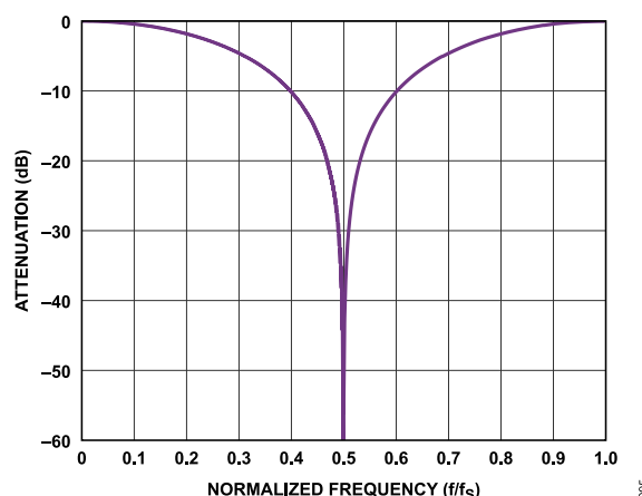
Figure 98. Sinc1 Filter Response, Decimate by 2
