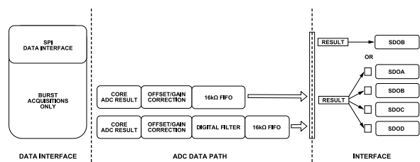
Figure 50. SPI Data Interface Data Path Options
