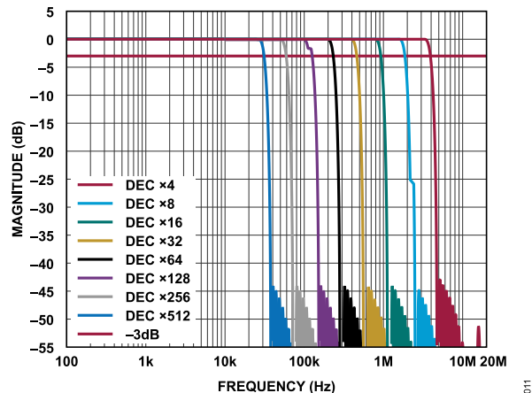
Figure 11. Sinc5 + Compensation Filter Response, f_s = 40 \text{ MHz}
