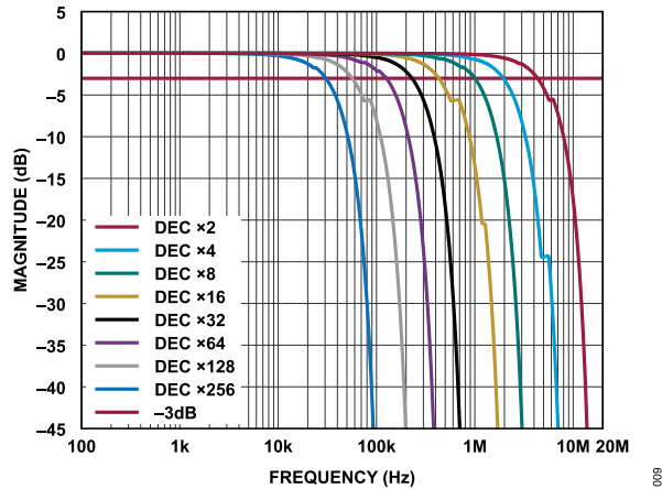
Figure 9. Sinc1 Filter Response, f_s = 40 \text{ MHz} (DEC x Means Decimate By)
