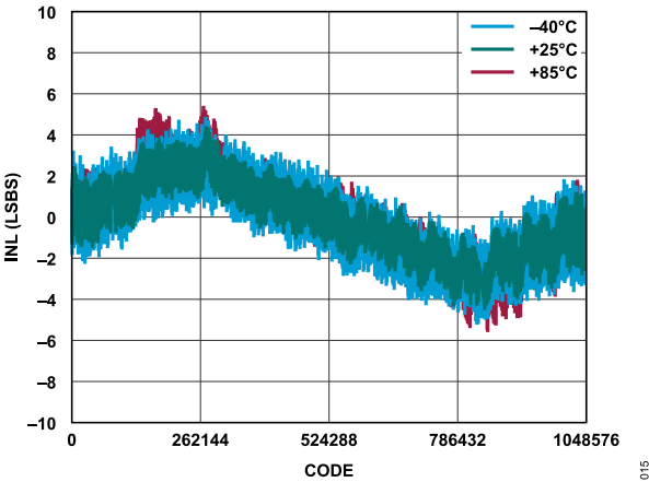
Figure 15. INL vs. Code for Various Temperatures, 40 MSPS
