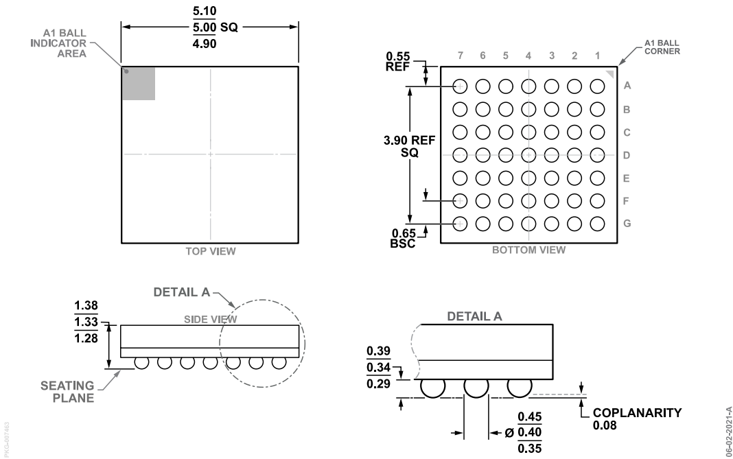
Figure 139. 49-Ball Chip Scale Package Ball Grid Array [CSP_BGA] (BC-49-8) Dimensions shown in millimeters
