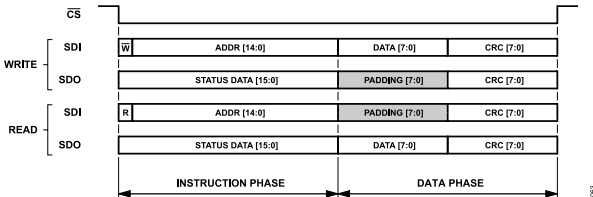
Figure 64. Long Instruction Mode, Data Status Enabled, CRC Enabled
