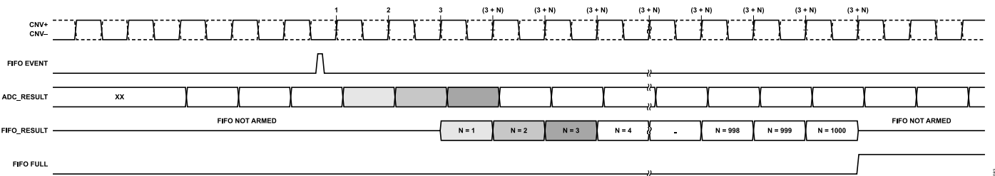
Figure 84. FIFO Data Capture Example, WATERMARK = 1000
