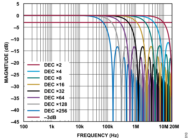
Figure 10. Sinc5 Filter Response, f_s = 40 \text{ MHz}
