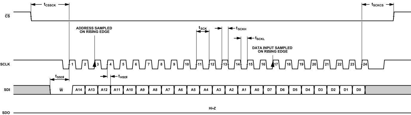
Figure 65. Configuration SPI Timing, Data Write Frame, 16-Bit Instruction Mode (Default)
