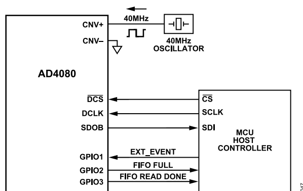
Figure 48. SPI Data Interface Clocking Example
