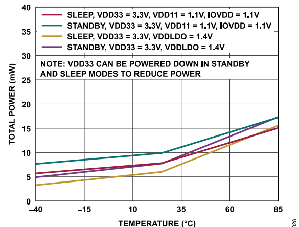
Figure 29. Total Power vs. Temperature in Sleep and Standby Modes
