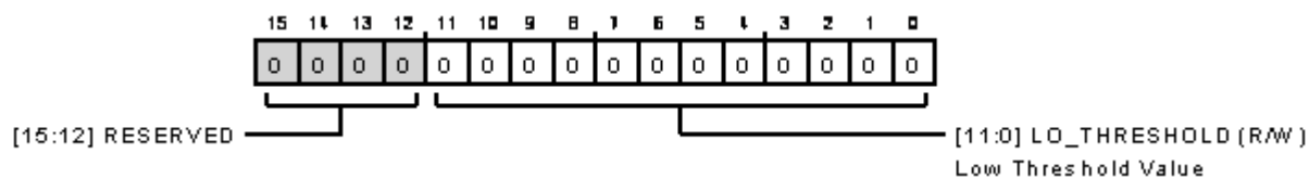
Figure 135. Event Detection Low Threshold Configuration Register
