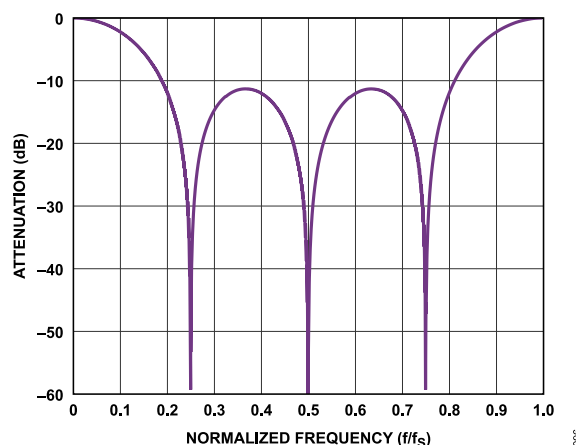
Figure 99. Sinc1 Filter Response, Decimate by 4
