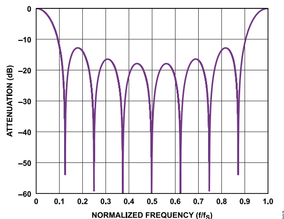
Figure 100. Sinc1 Filter Response, Decimate by 8
