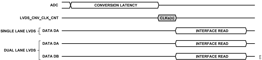
Figure 79. LVDS Data Transfer Latency
