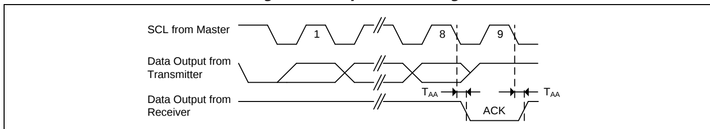
Figure 5-2. Output Acknowledge
