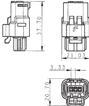
Female housing - full shroud
