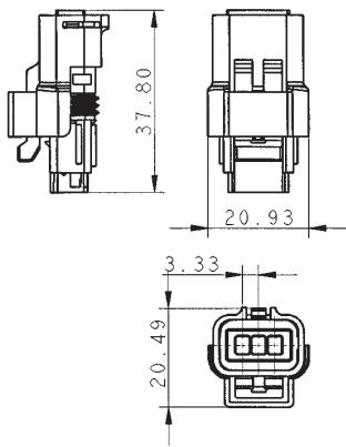
Male housing
