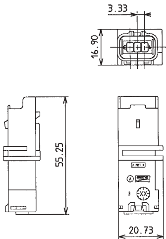
Male housing
