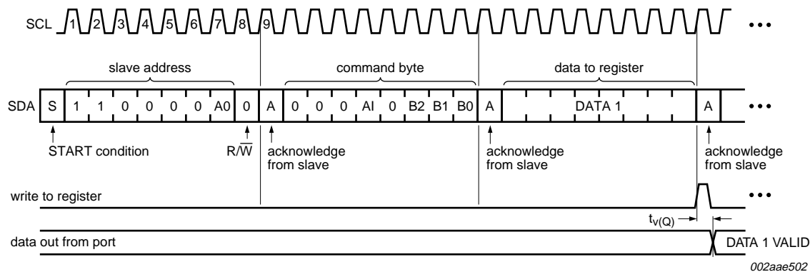
Fig 10. Write to register
