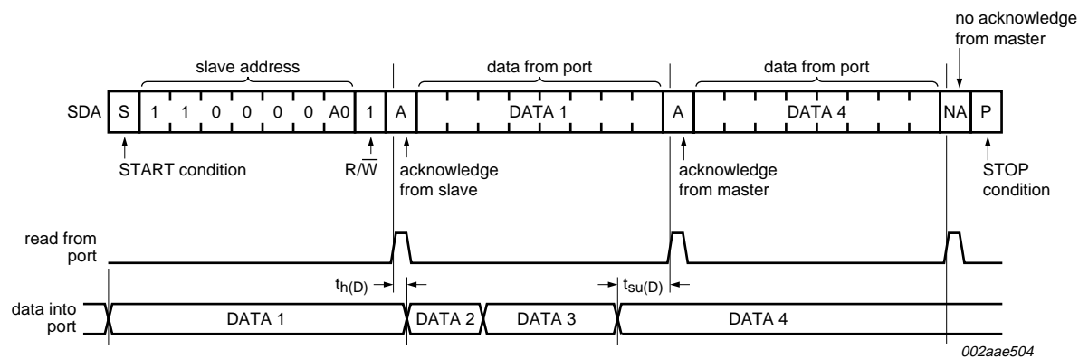
Fig 12. Read Input port register
