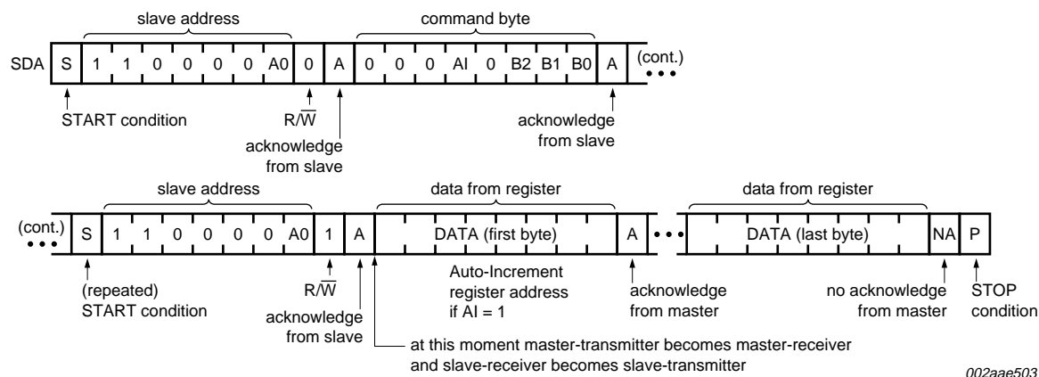
Fig 11. Read from register
