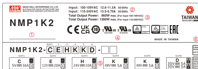
Figure 2-2. NMP1K2 Product Label
