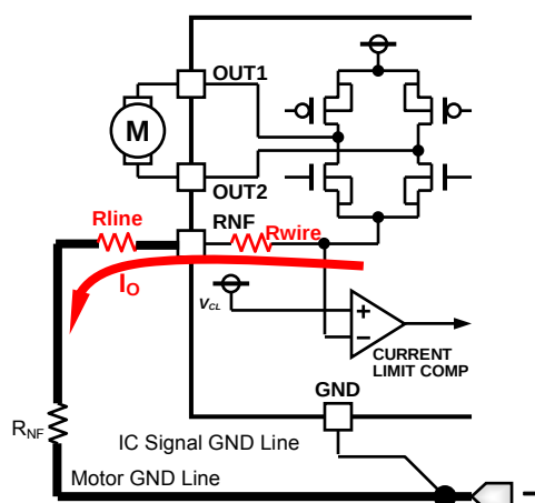
Figure 41. Current limit setting and GND line
