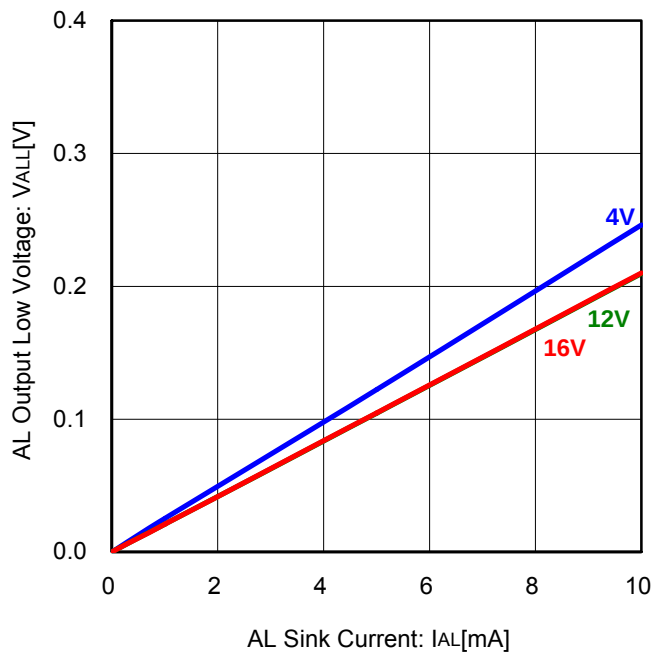
Figure 13. AL Output Voltage vs AL Sink Current ( T_a=25^\circ C )
