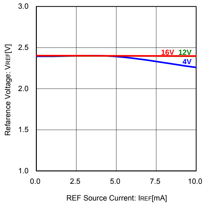
Figure 18. Reference Voltage vs REF Source Current ( T_a=25^{\circ}C )
