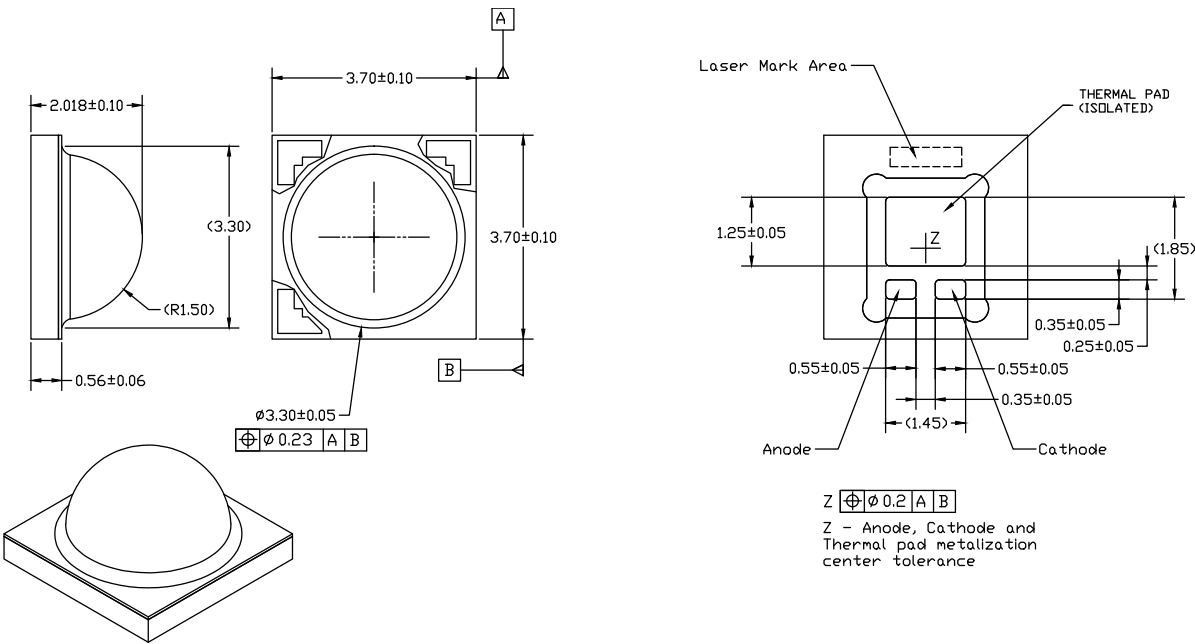
Figure 9. Mechanical dimensions for LUXEON TX.
