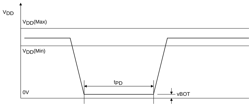
Figure 19 Power-down Timing
