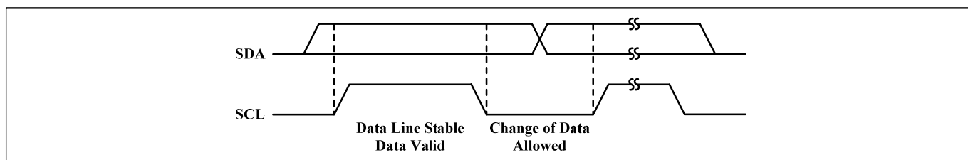
Figure 5 Bit Transfer
