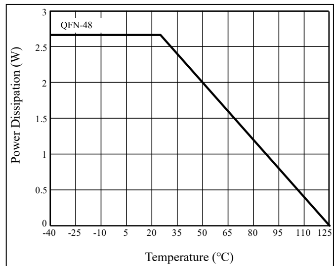
Figure 18 Dissipation Curve
