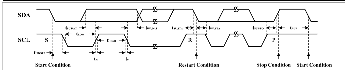
Figure 4 Interface Timing
