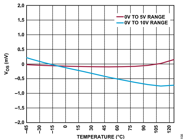
Figure 9. Unipolar Offset Error ( V_{OS} ) vs. Temperature
