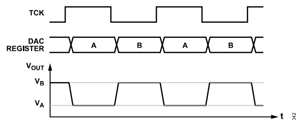
Figure 54. TCK Timing
