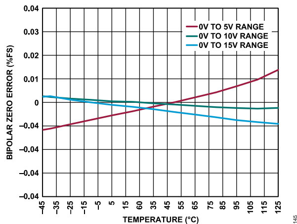
Figure 35. Bipolar Zero Error vs. Temperature
