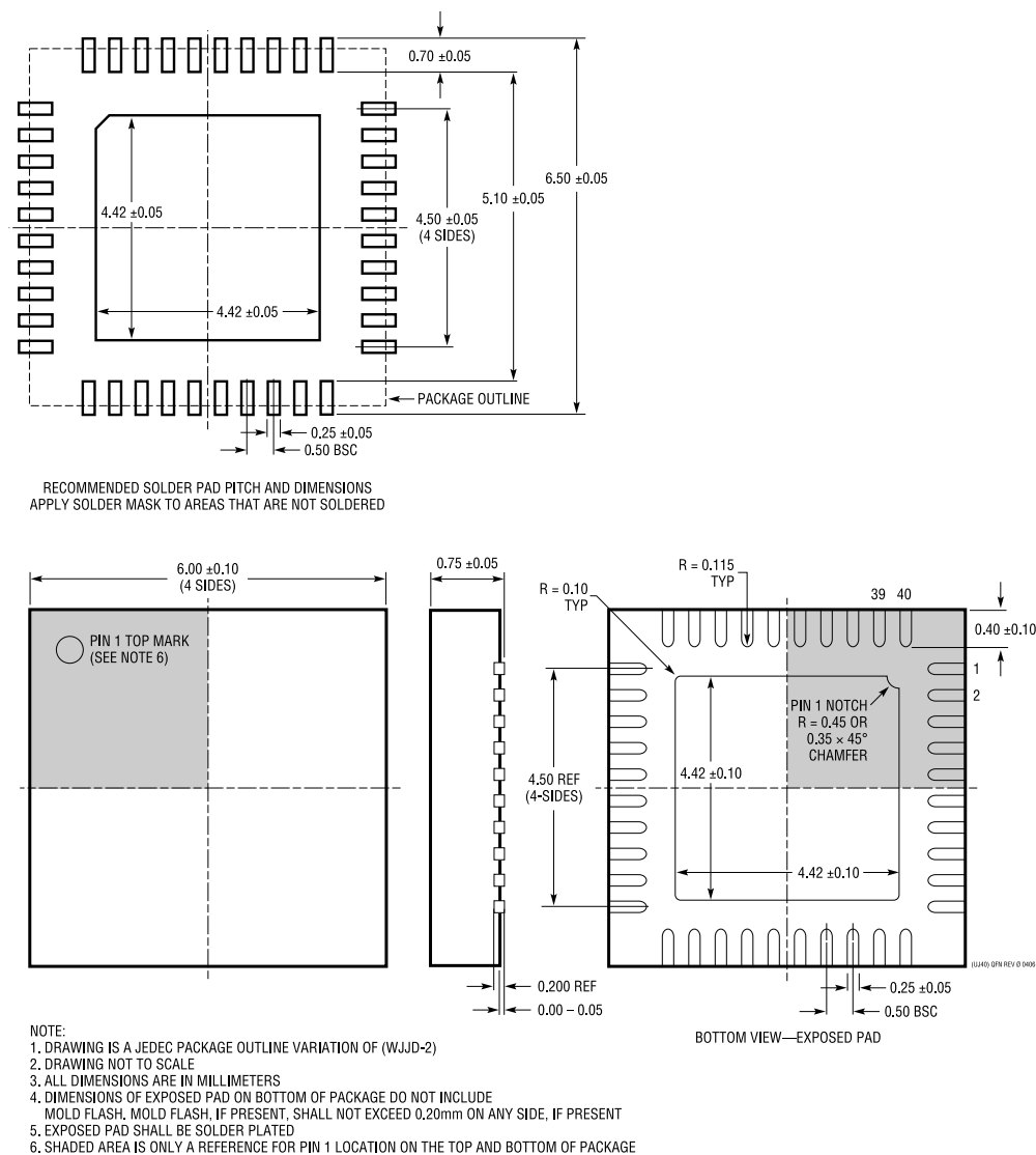
Figure 61. 40-Lead Lead Frame Chip Scale Package [LFCSP]
