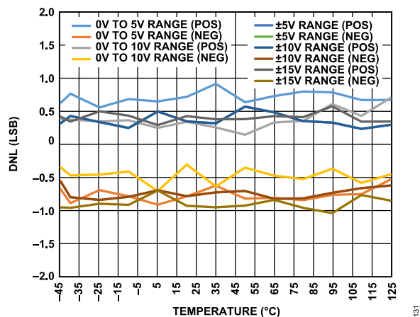
Figure 29. LTC2688-16 DNL vs. Temperature
