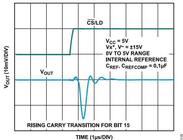
Figure 16. Glitch Impulse
