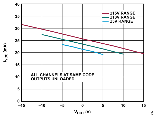
Figure 13. I_{VCC} vs. V_{OUT}
