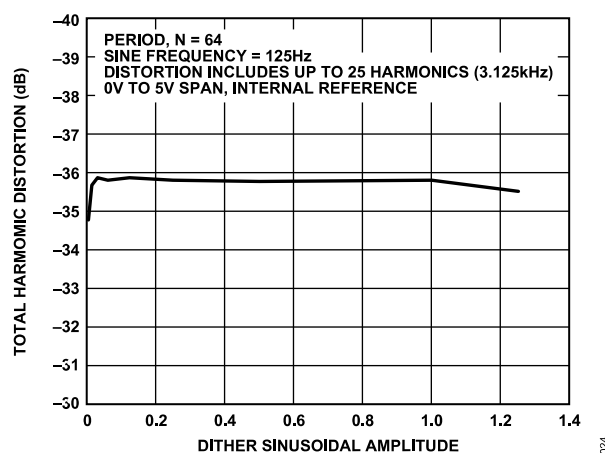
Figure 22. Total Harmonic Distortion (THD) vs. Dither Sinusoidal Amplitude
