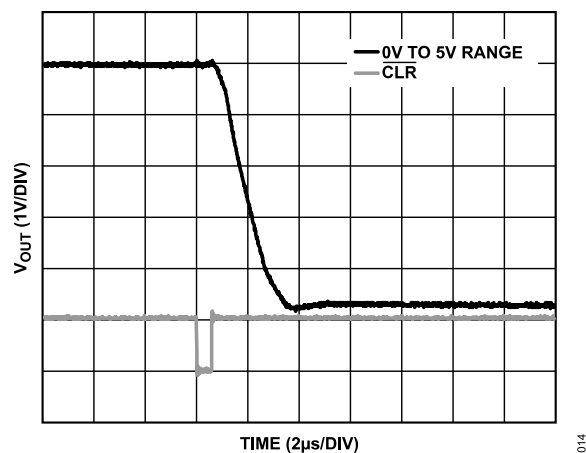
Figure 14. Hardware \overline{CLR} to Zero Scale
