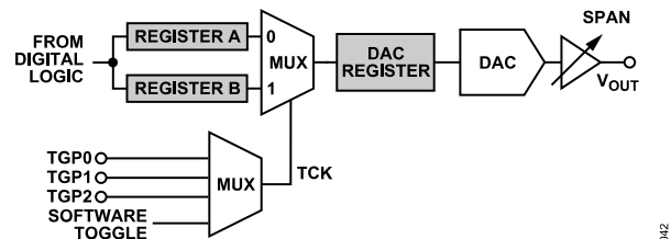
Figure 53. Toggle Operation
