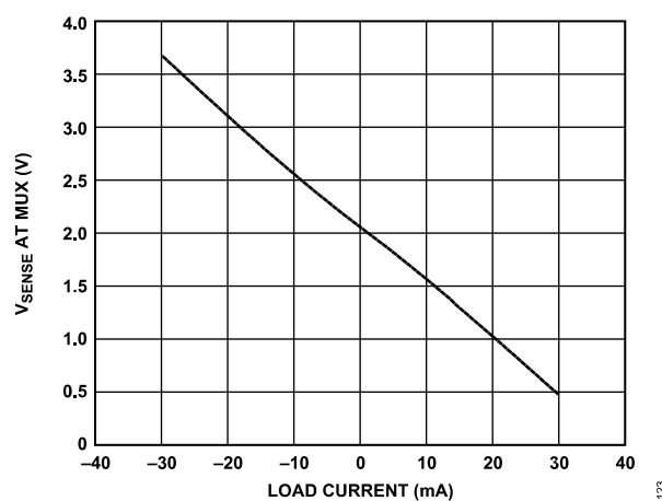
Figure 21. V_{SENSE} at MUX vs. Load Current
