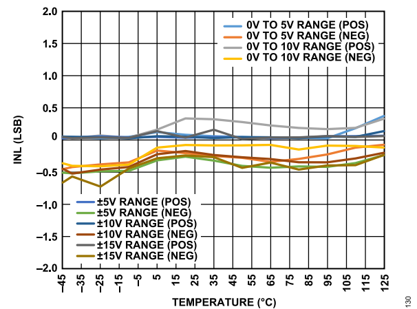
Figure 28. LTC2688-16 INL vs. Temperature
