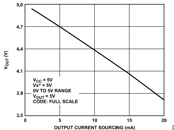
Figure 10. V_{OUT} vs. Output Current Sourcing
