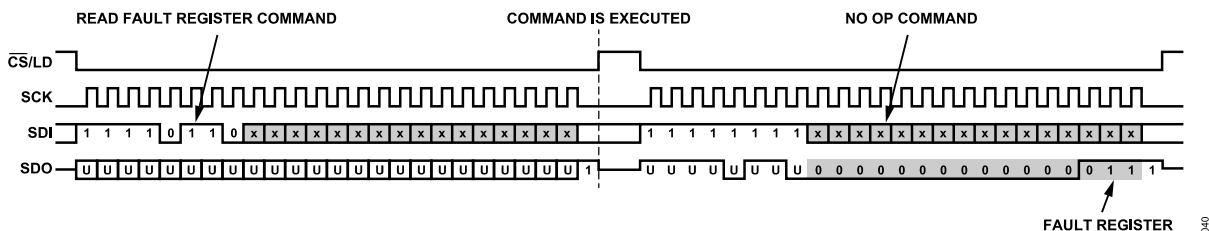
Figure 50. Typical Read Command Sequence for 24-Bit Words
