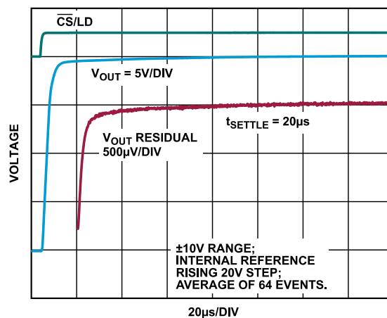
Figure 40. Settling Time, 20 V
