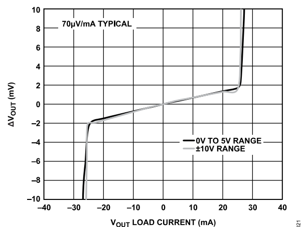
Figure 19. \Delta V_{OUT} vs. V_{OUT} Load Current
