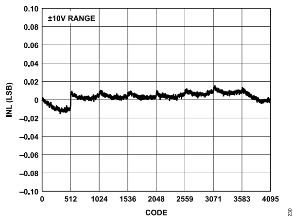
Figure 30. LTC2688-12 INL vs. Code
