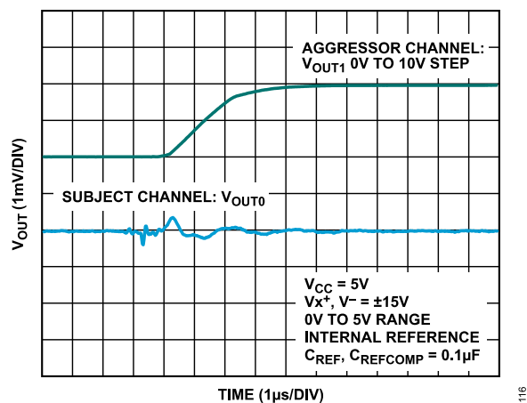
Figure 17. DAC to DAC Crosstalk
