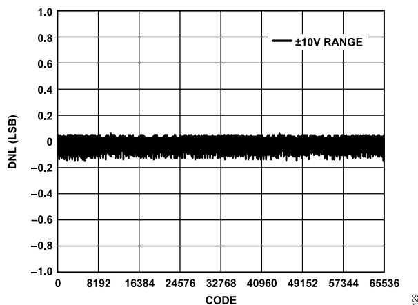
Figure 27. LTC2688-16 DNL vs. Code
