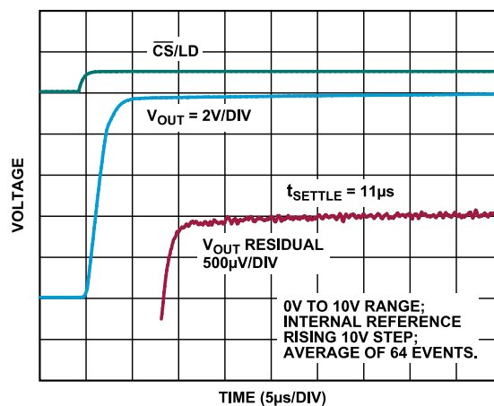
Figure 38. Settling Time, 10 V
