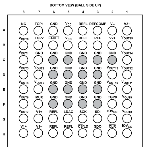
Figure 4. WLCSP Pin Configuration
