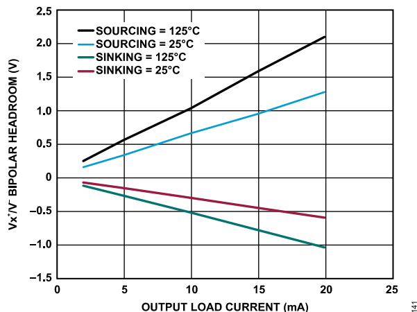
Figure 45. V_{x+}/V_{-} Bipolar Headroom vs. Output Load Current
