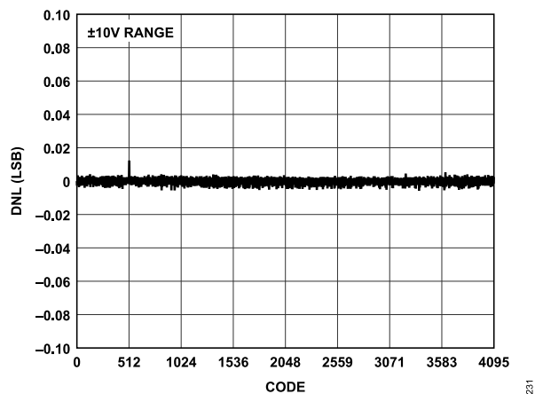
Figure 31. LTC2688-12 DNL vs. Code
