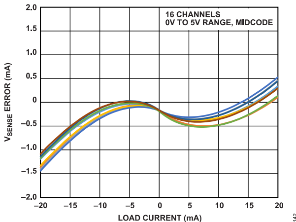
Figure 46. V_{SENSE} Error vs. Load Current from Equation 5
