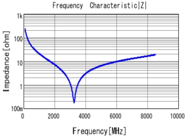
■ GCQ1555C1H6R9WB01 |Z| DC0V, 25degC
