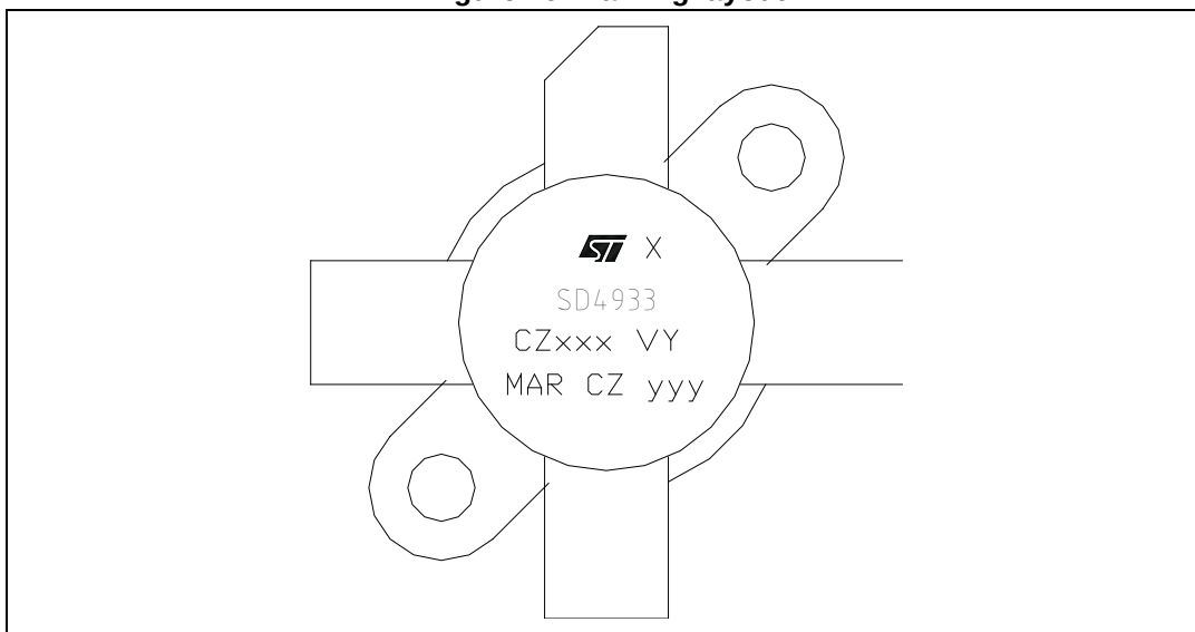
Figure 16. Marking layout
