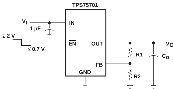
Figure 28. TPS75701 Adjustable LDO Regulator Programming
