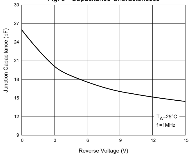
Fig. 3 - Capacitance Characteristics
