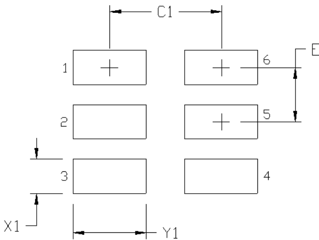
Figure 6.2. Si566 (3.2×5 mm) PCB Land Pattern
