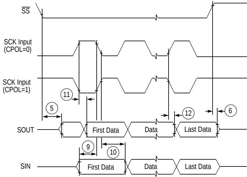
Figure 33. DSPI classic SPI timing — slave, CPHA = 1
