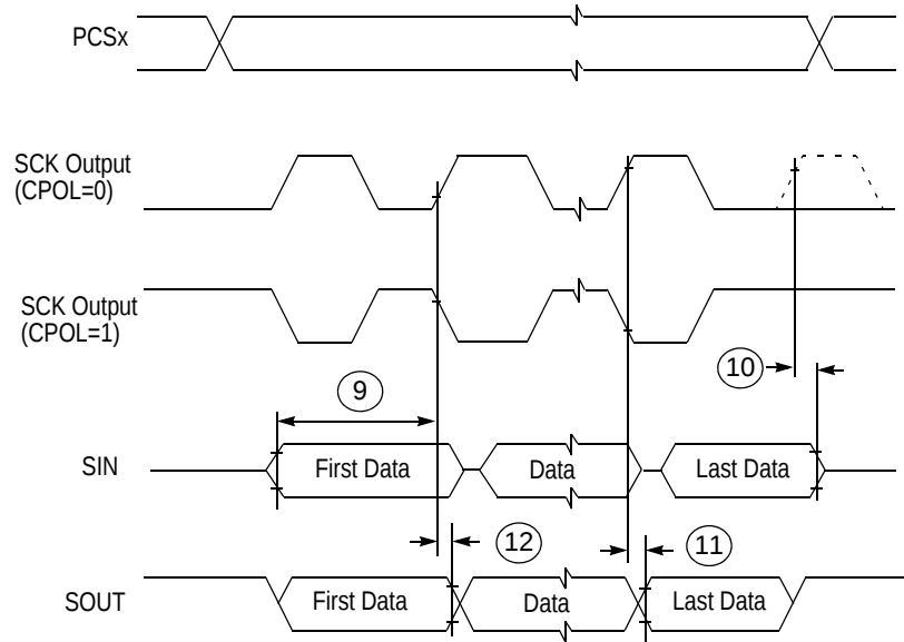
Figure 35. DSPI modified transfer format timing — master, CPHA = 1
