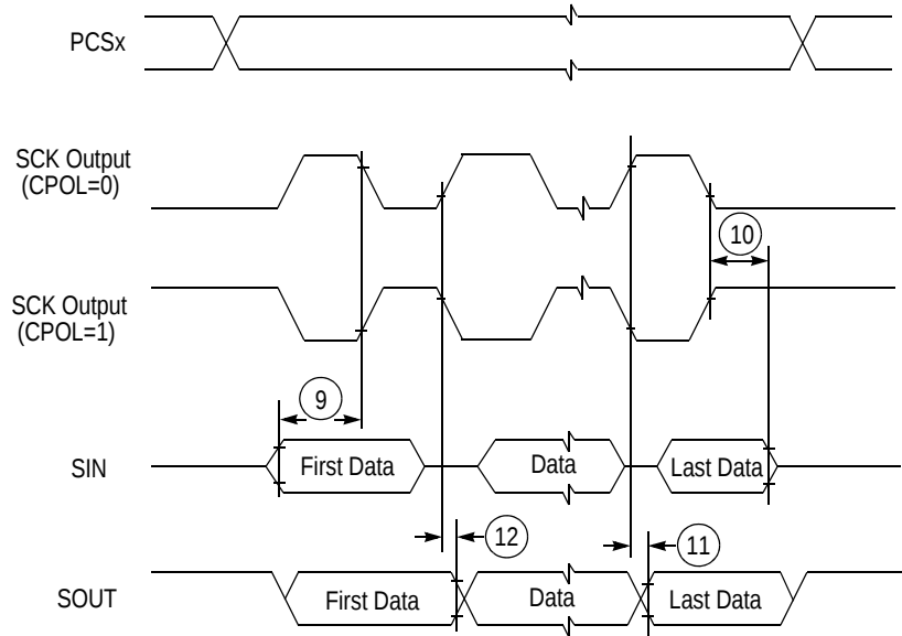
Figure 31. DSPI classic SPI timing — master, CPHA = 1
