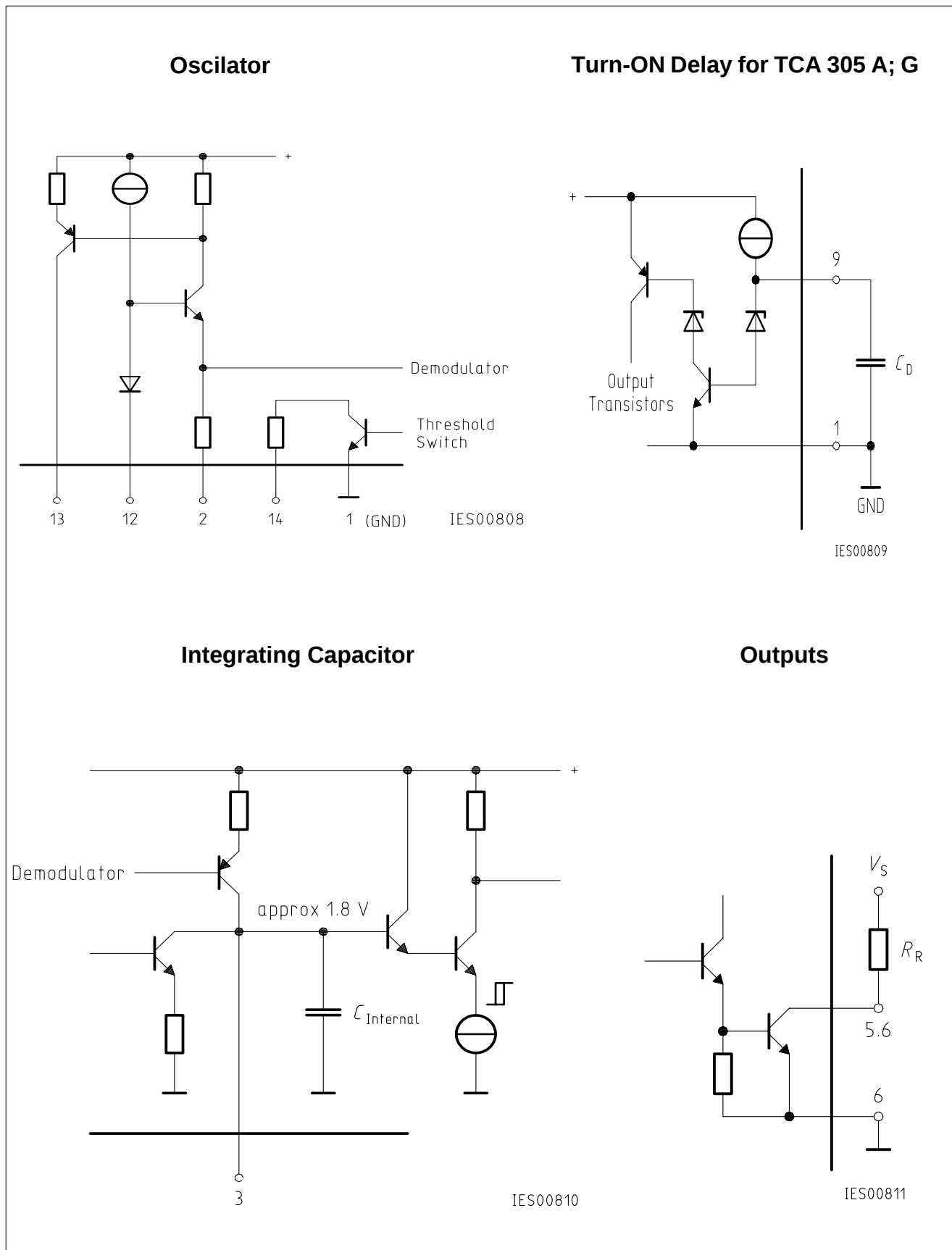
Schematic Circuit Diagram
