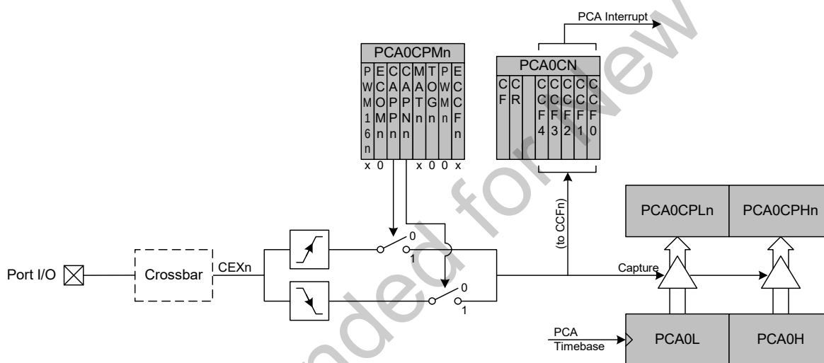
Figure 23.4. PCA Capture Mode Diagram
