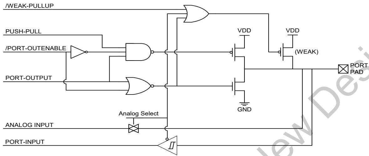
Figure 18.2. Port I/O Cell Block Diagram
