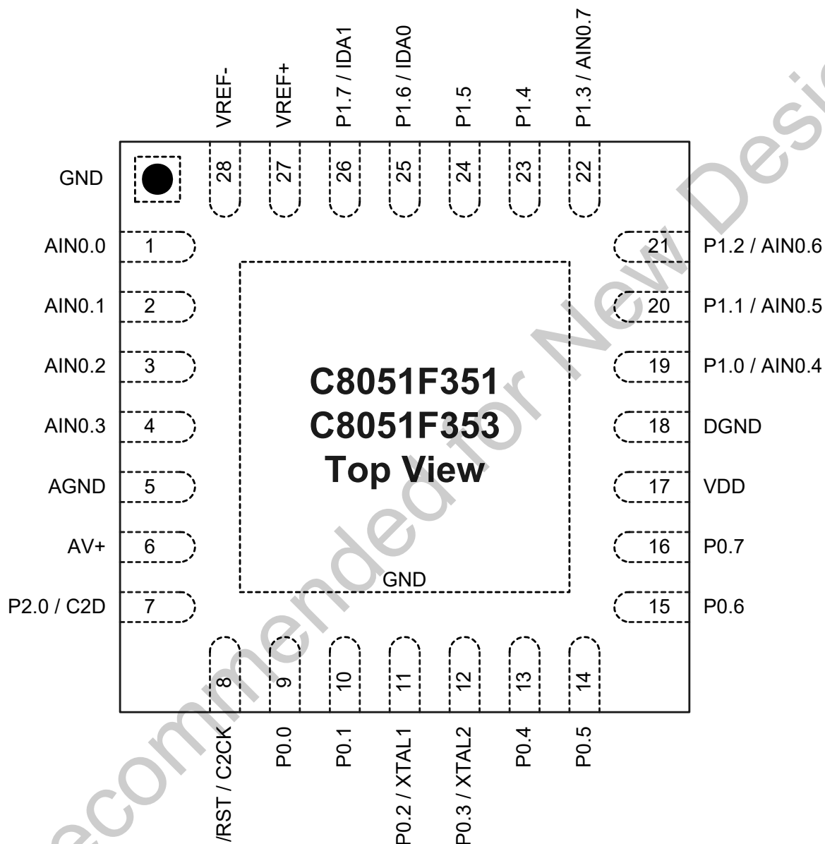
Figure 4.2. QFN-28 Pinout Diagram (Top View)
