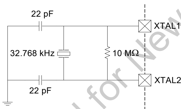
Figure 17.2. 32.768 kHz External Crystal Example
