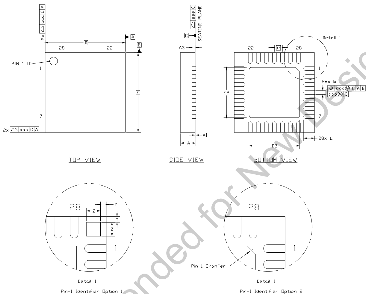
Figure 4.4. QFN-28 Package Drawing
