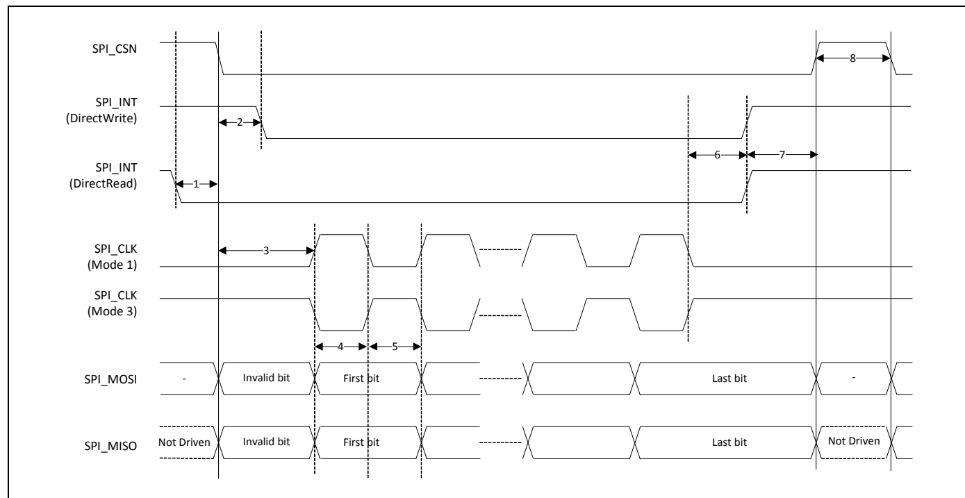
Figure 12. SPI Timing, Mode 1 and 3
