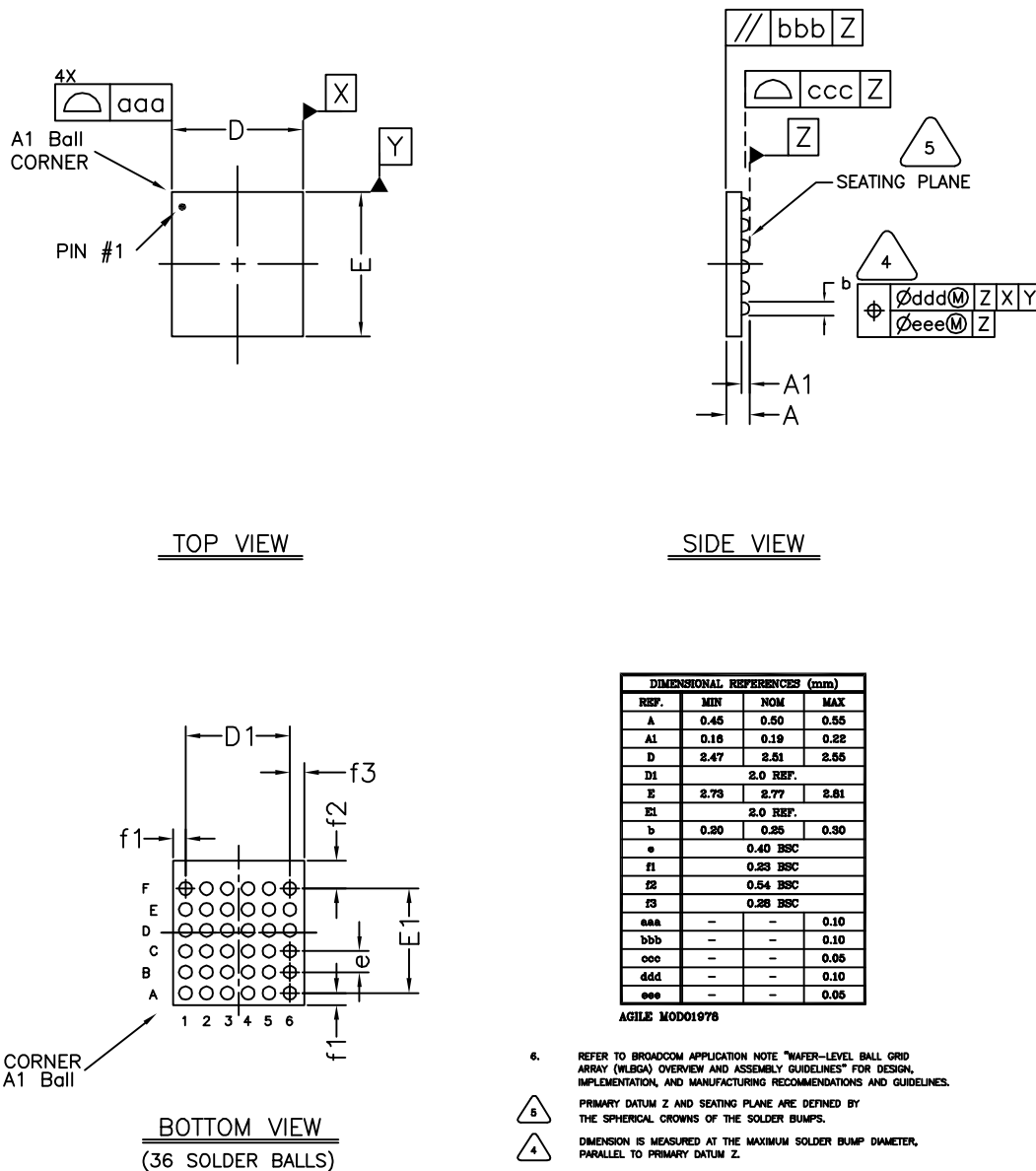
Figure 21. CYW20707 36-pin WLBGA Package (2.8 mm x 2.5 mm)
