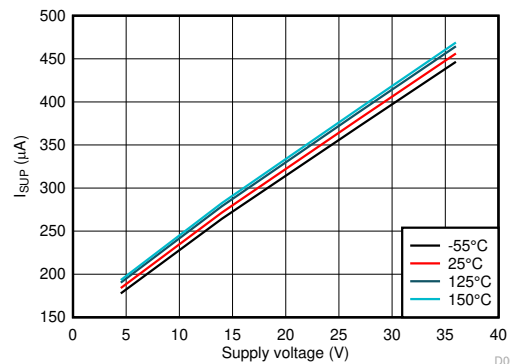
Figure 7-4. I_{SUP} Recessive vs V_{SUP} and Temperature
