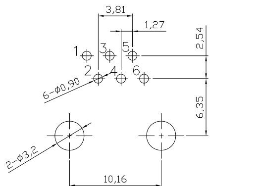
PC Board Layout Component Side Shown(6P4C)
