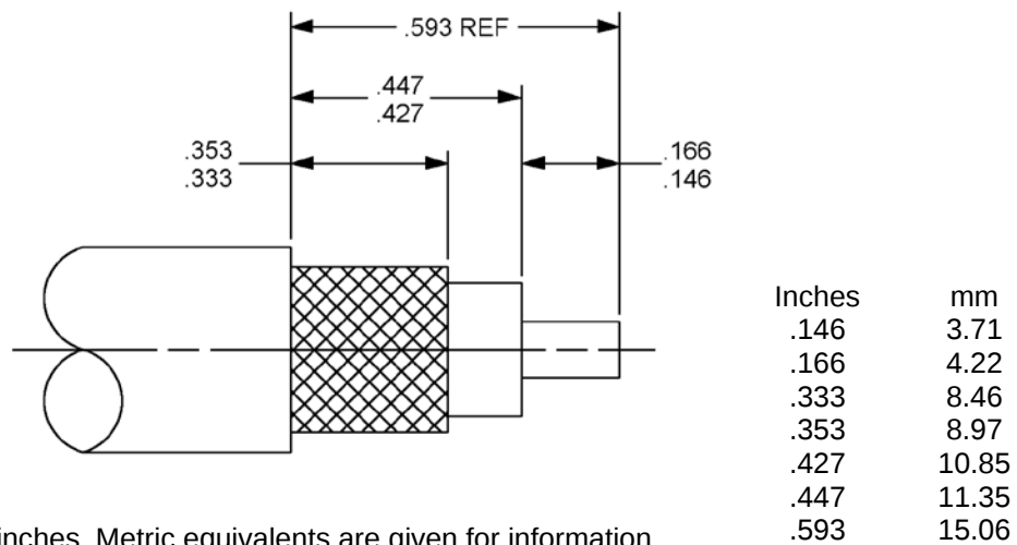
FIGURE 4. Cable stripping dimensions for field replaceable connectors.
