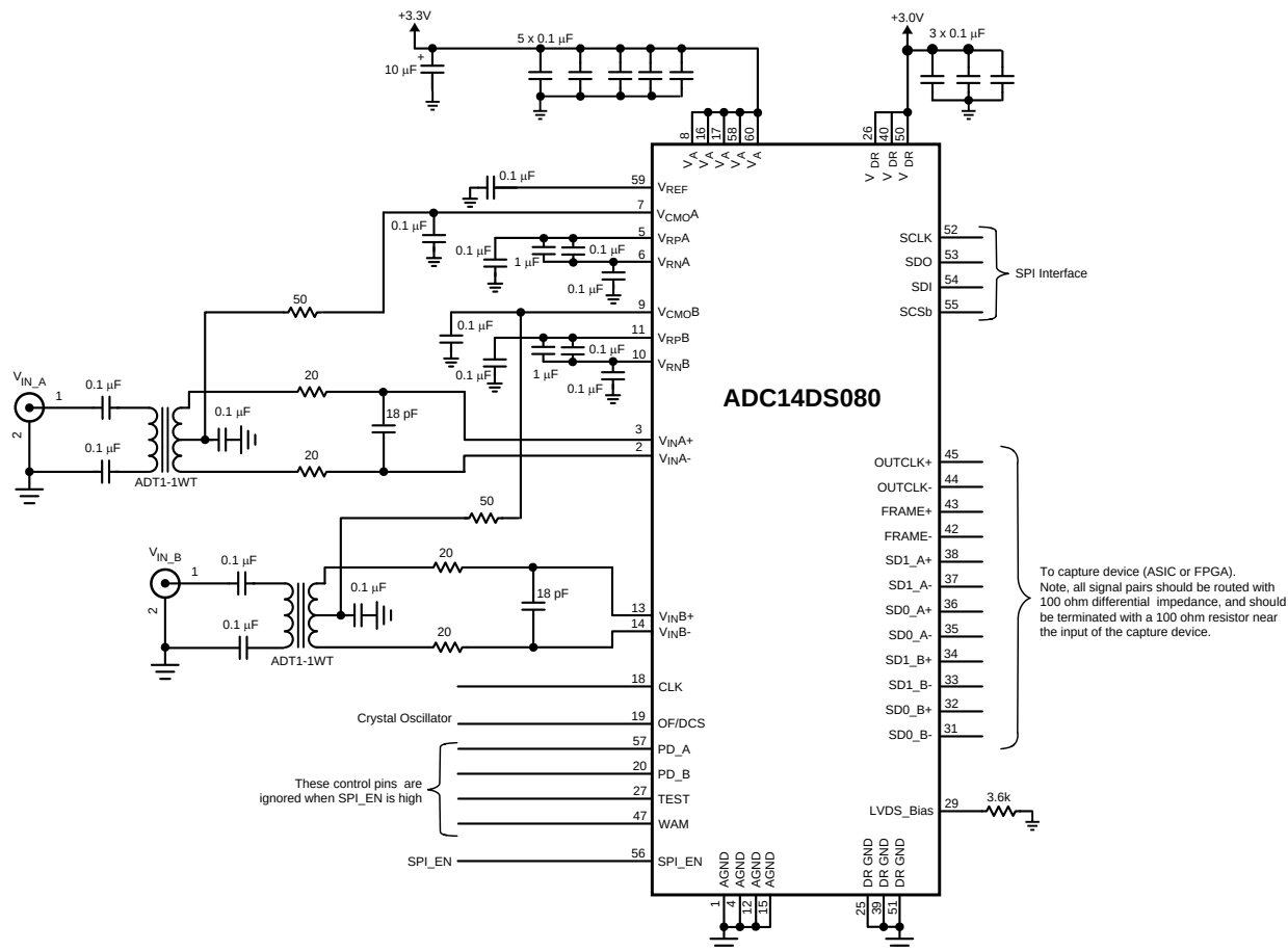
Figure 21. Application Circuit
