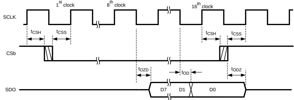
Figure 23. Read Timing
