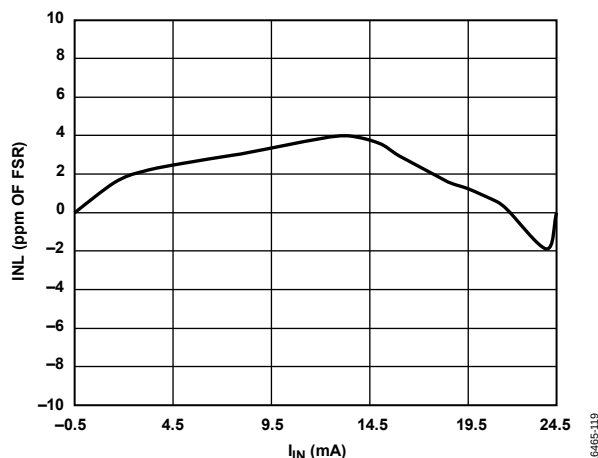
Figure 19. Integral Nonlinearity (INL) vs. Input (Current Input)
