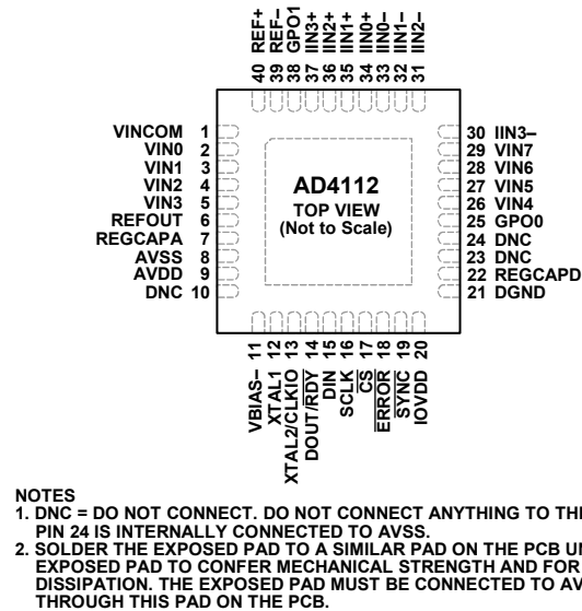
Figure 4. Pin Configuration
