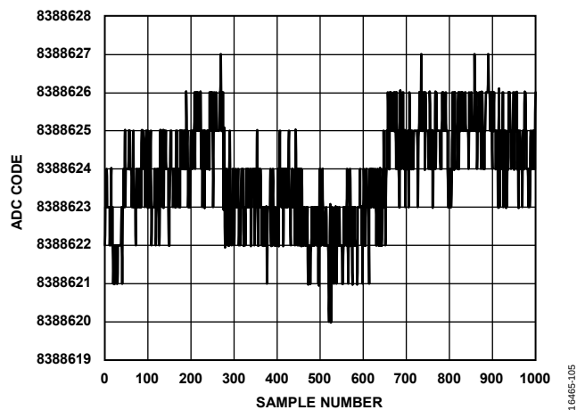
Figure 5. Noise (Voltage Input, Output Data Rate = 1.25 SPS)
