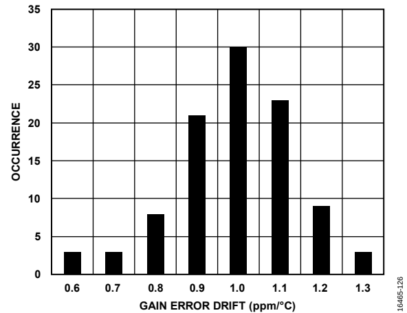
Figure 26. Gain Error Drift Distribution Histogram (Voltage Input)
