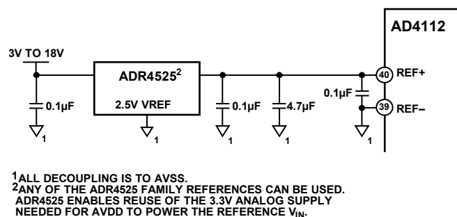
Figure 39. ADR4525 Connected to AD4112 REF± Pins
