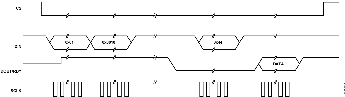
Figure 56. Single Conversion Mode
