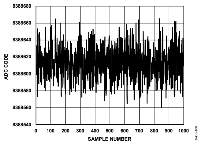
Figure 6. Noise (Voltage Input, Output Data Rate = 2.5 kSPS)
