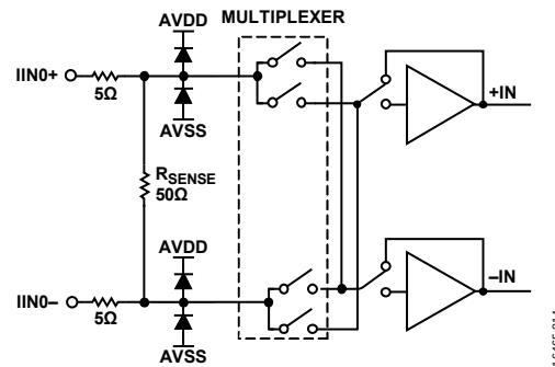
Figure 37. Simplified Current Input Circuit
