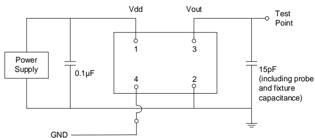
Figure 2. Test Circuit [10]
