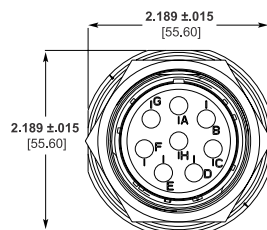
Receptacle, Shell Size 25 38999 Style Arrangement 8Q8, RR-RR Jam Nut Part No. 2157628
