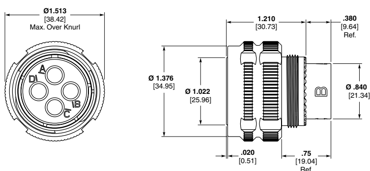
Plug, Shell Size 19 Arrangement 4Q4, RR-RR Part No. 1811902
