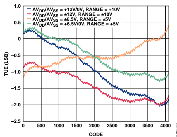
Figure 37. AD5722 Total Unadjusted Error vs. Code
