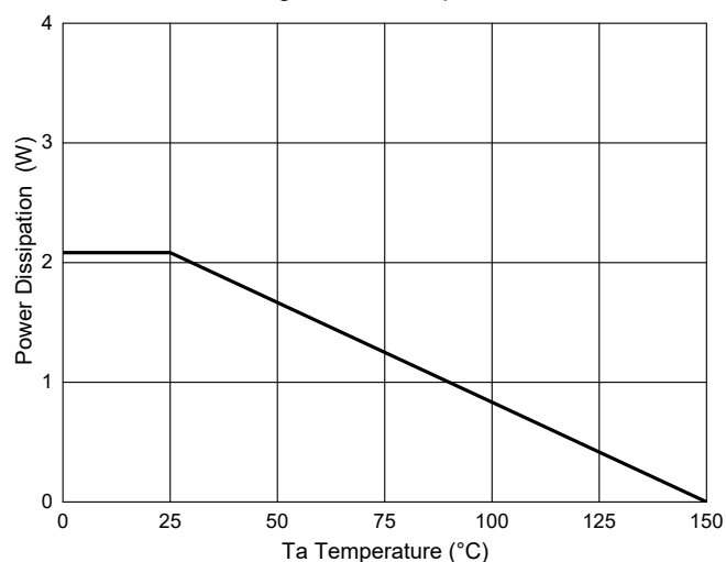
Fig.11 - PD Dissipation
