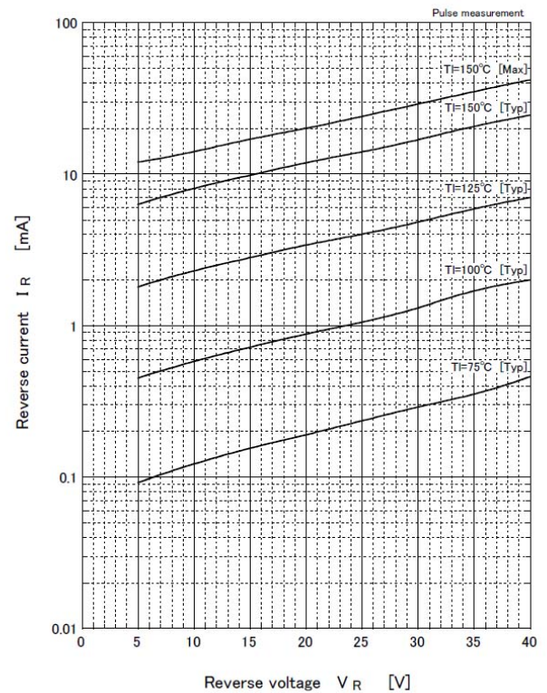
Reverse current
