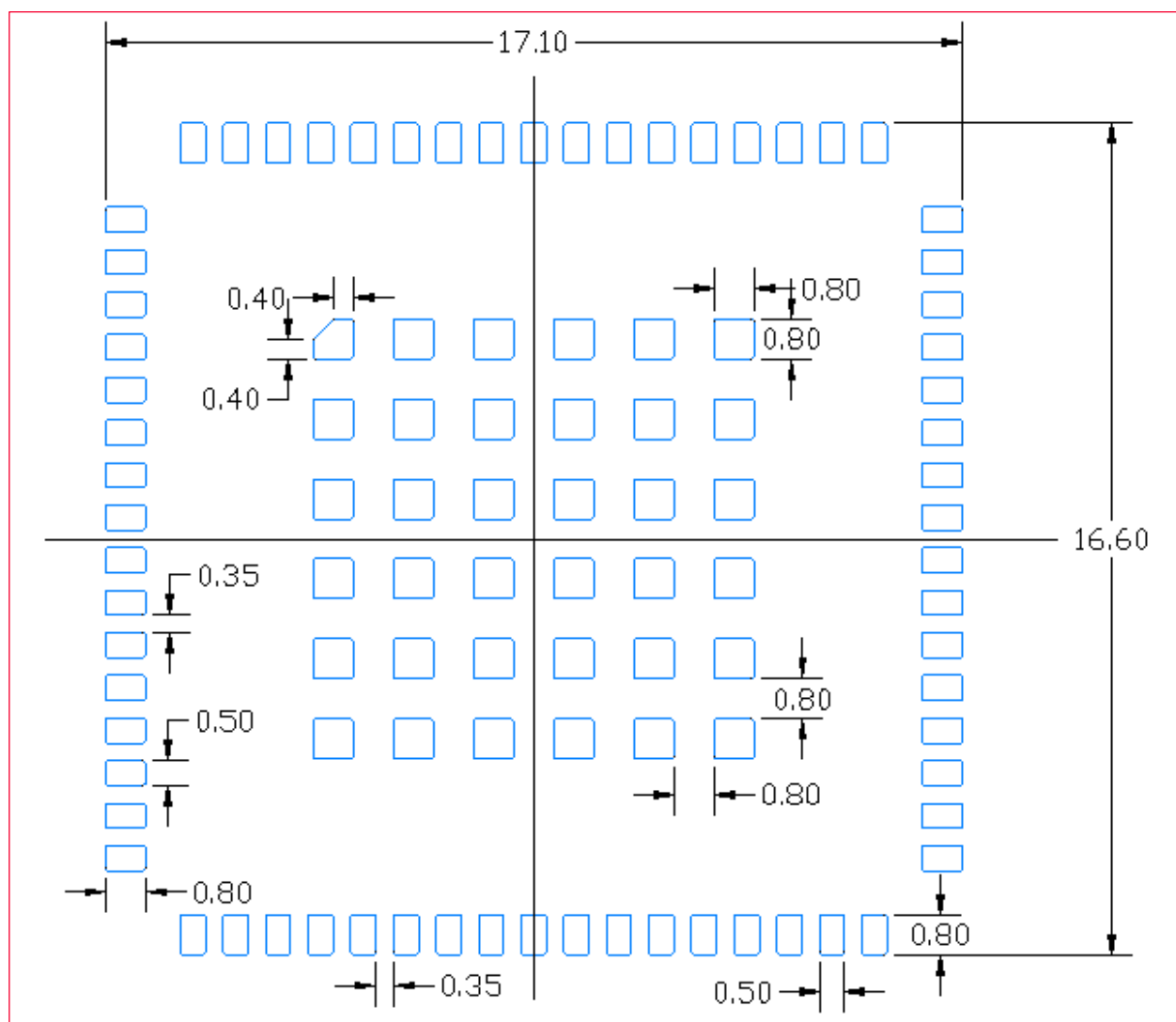
Figure 7: Land Pattern
