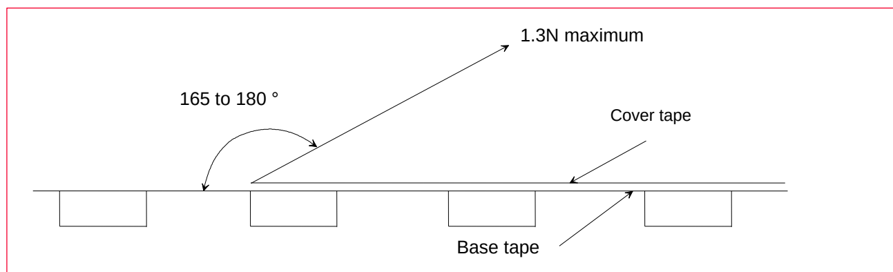
Figure 16: Peeling Force
