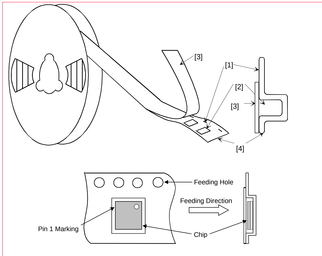
Figure 14: Taping Diagrams
