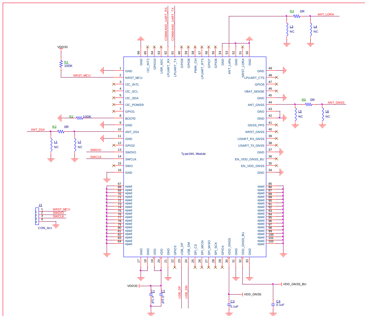
Figure 8: Reference Circuit
