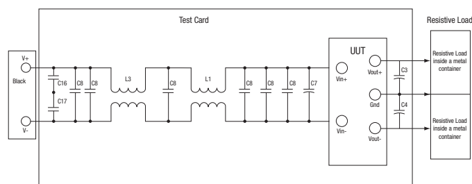
Figure 4. Conducted Emissions Test Circuit
