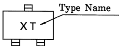
Fig. 9.3 Marking RN1416
