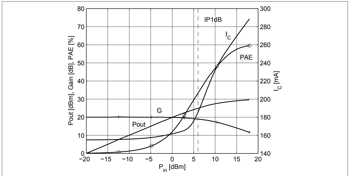
Figure 20 P_{out} , Gain, I_C , PAE vs. P_{in} at V_{CE} = 5\text{ V} , I_{Cq} = 155\text{ mA} , f = 0.9\text{ GHz} , Z_I = Z_{opt}
