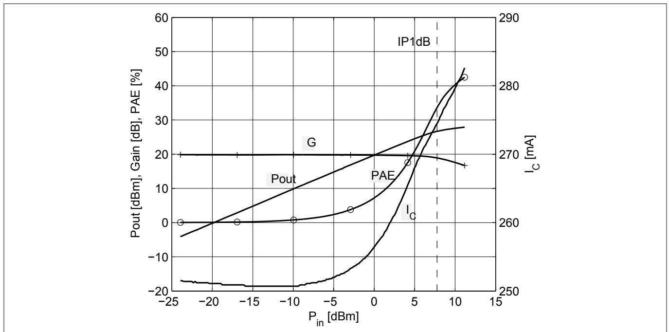
Figure 21 P_{out} , Gain, I_C , PAE vs. P_{in} at V_{CE} = 5\text{ V} , I_{Cq} = 250\text{ mA} , f = 0.9\text{ GHz} , Z_I = Z_{opt}
