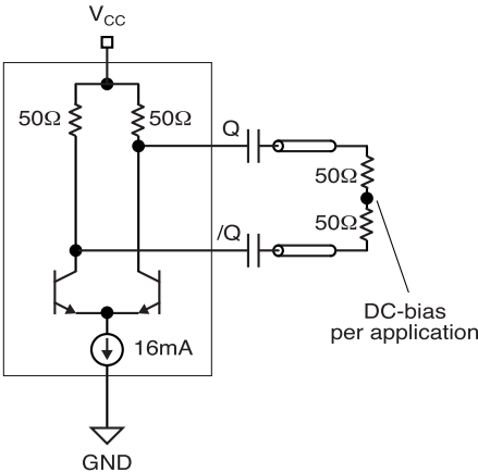
Figure 5. CML AC-Coupled Termination
