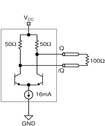
Figure 4. CML DC-Coupled
