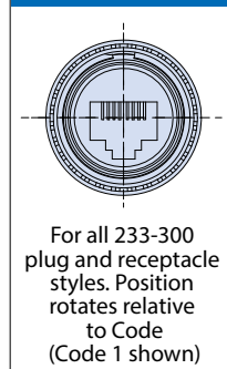
Rear View
